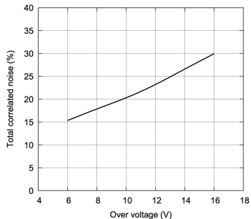
Figure 11: Total Correlated Noise vs. Overvoltage
